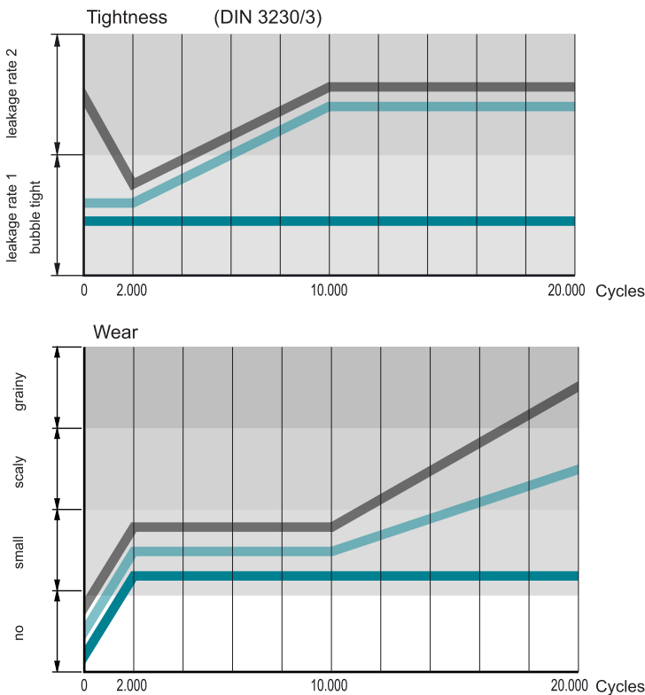
Endurance test (tightness)
